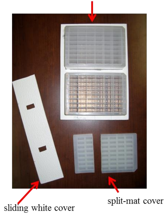
Figure 1. 48-well-plate-transfer-guide
